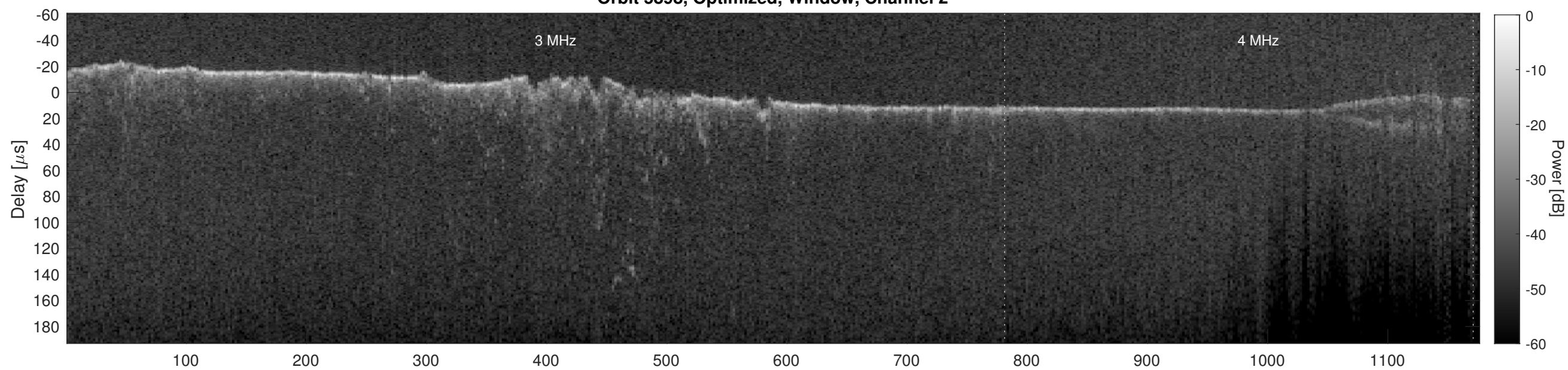
Orbit 5898, Cluttergram
