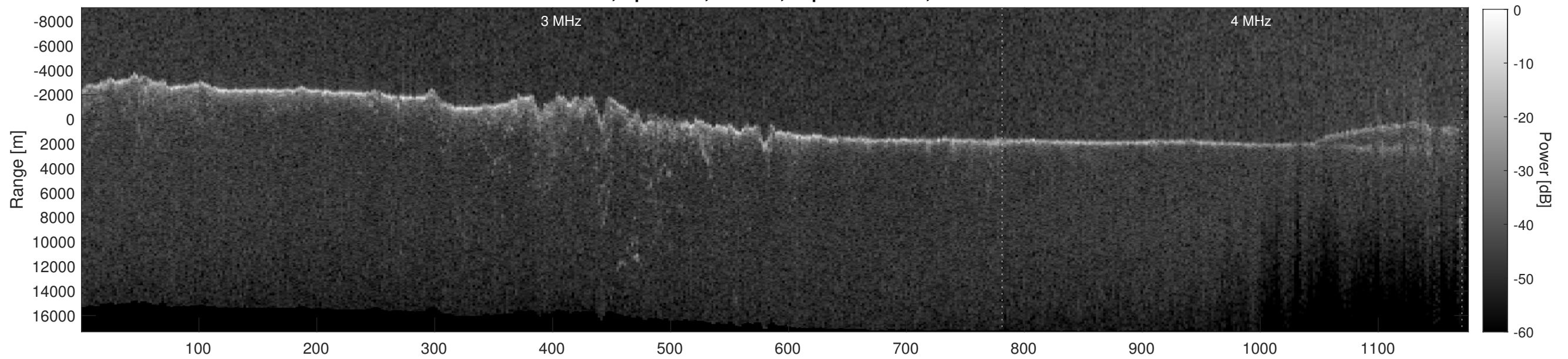
Orbit 5898, Depth-Corrected Cluttergram
