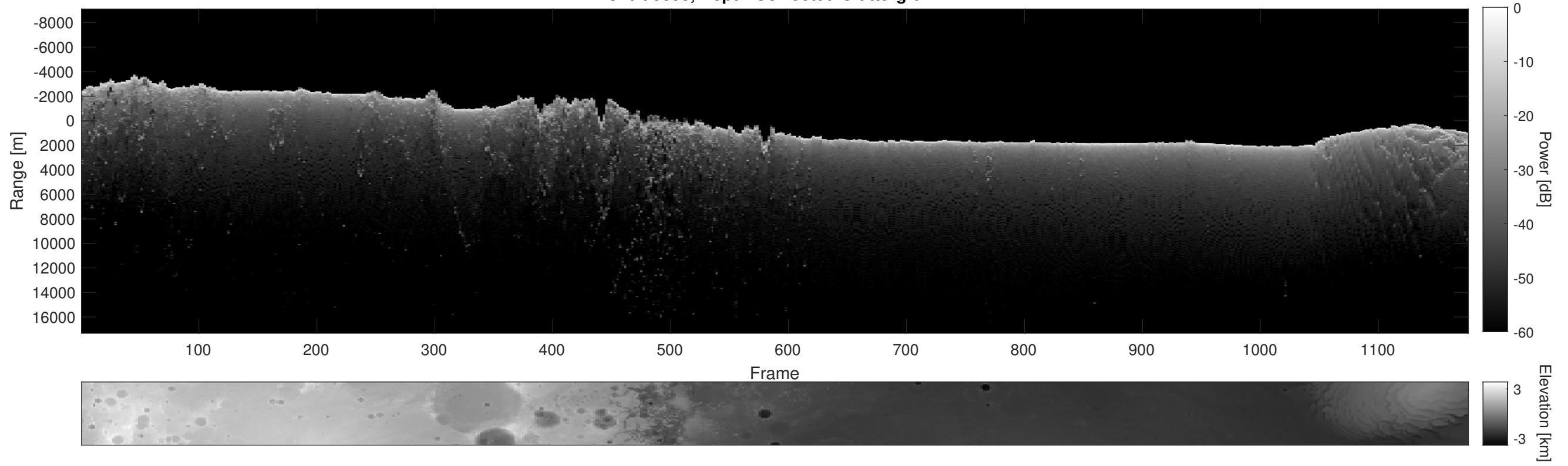
Orbit 5898, Depth-Corrected Cluttergram
