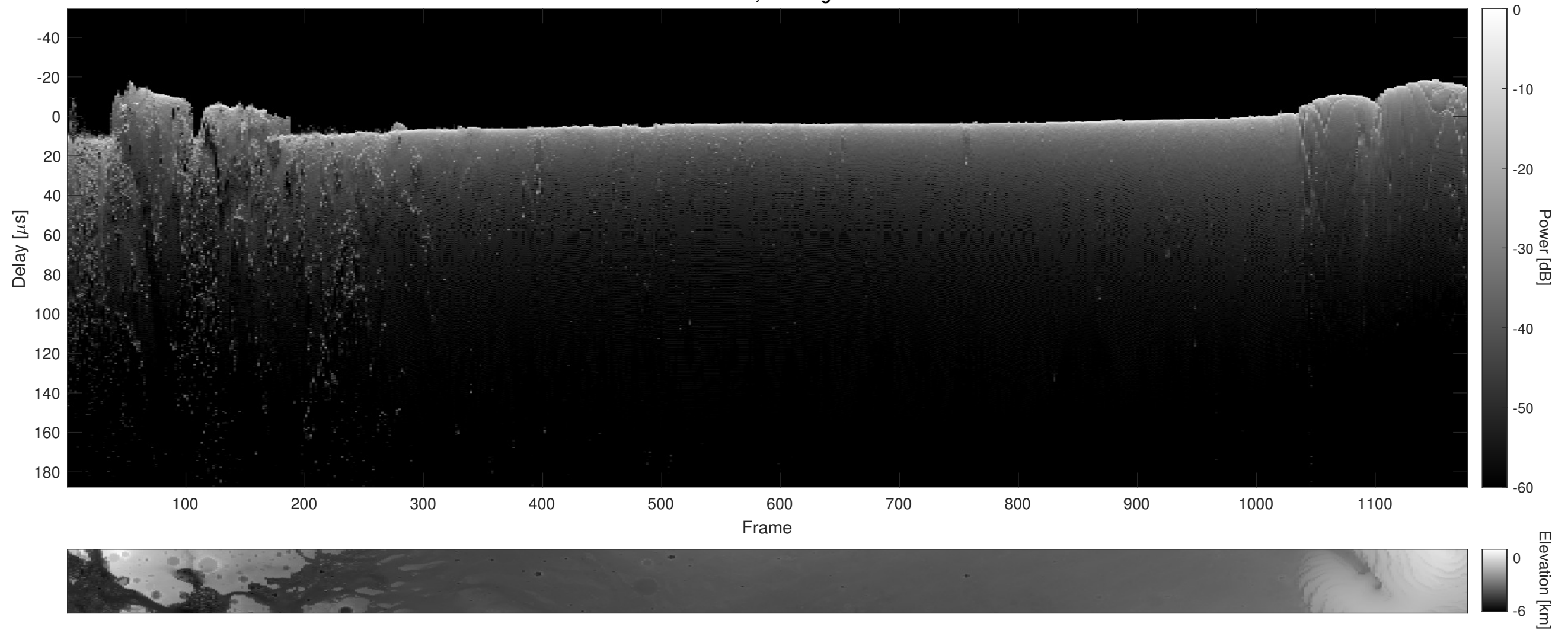
Orbit 5899, Cluttergram
