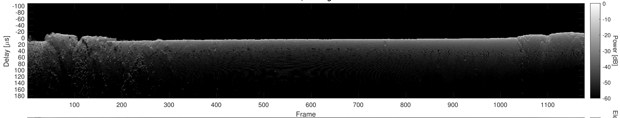
Orbit 5899, Cluttergram
