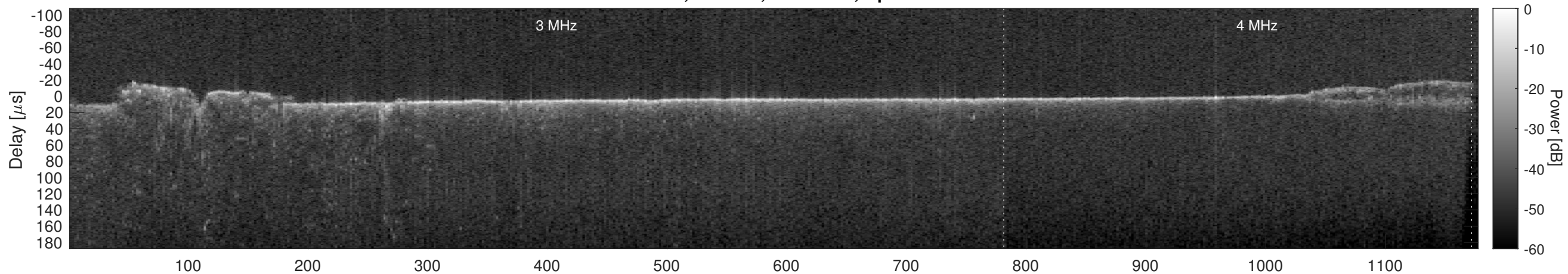
Orbit 5899, Cluttergram
