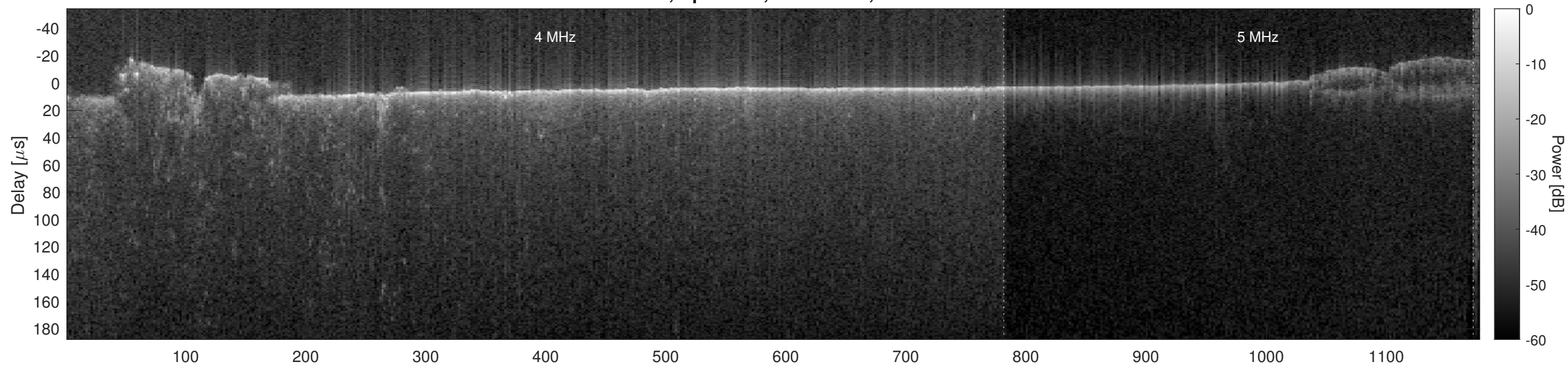
Orbit 5899, Optimized, No Window, Channel 2
