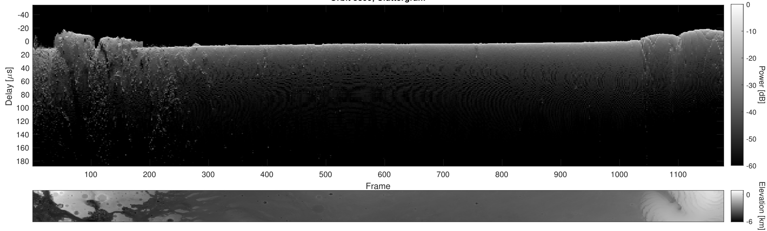
Orbit 5899, Cluttergram
