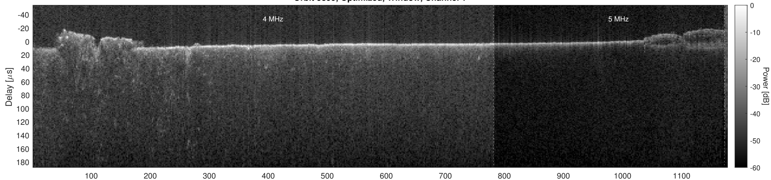
Orbit 5899, Optimized, Window, Channel 2
