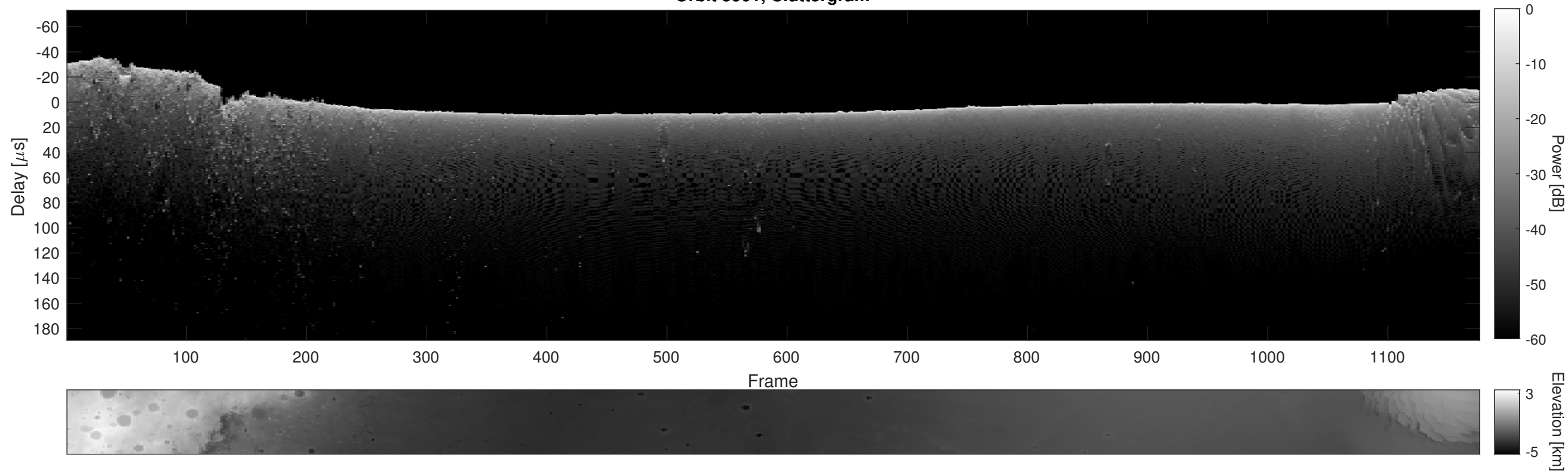
Orbit 5901, Cluttergram
