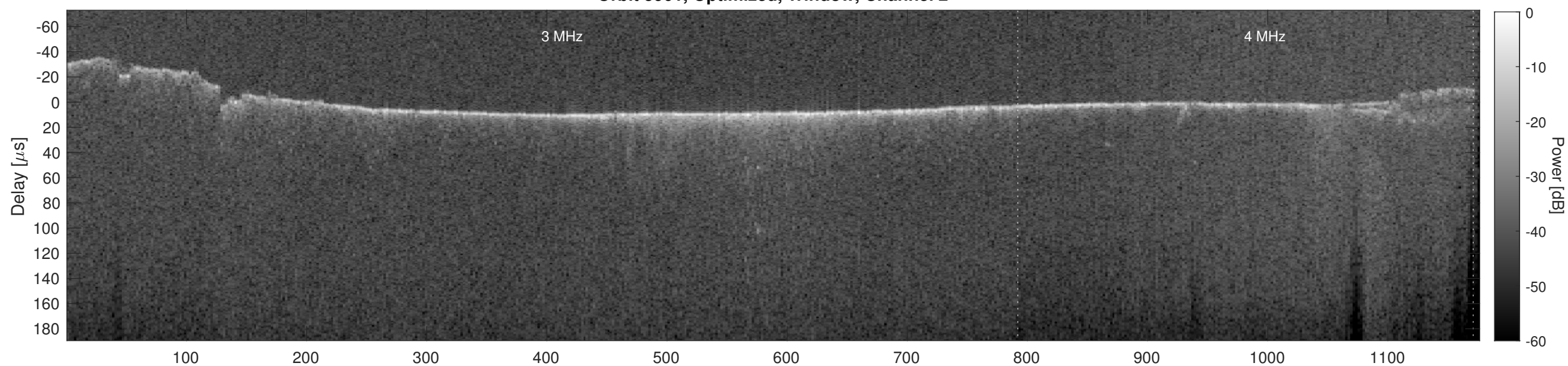
Orbit 5901, Cluttergram
