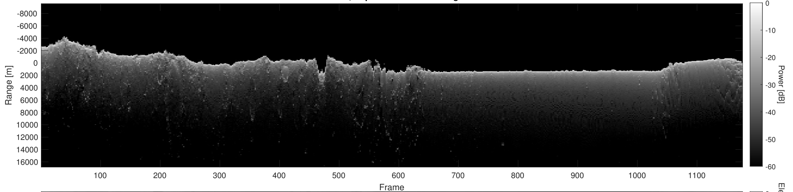
Orbit 5902, Depth-Corrected Cluttergram
