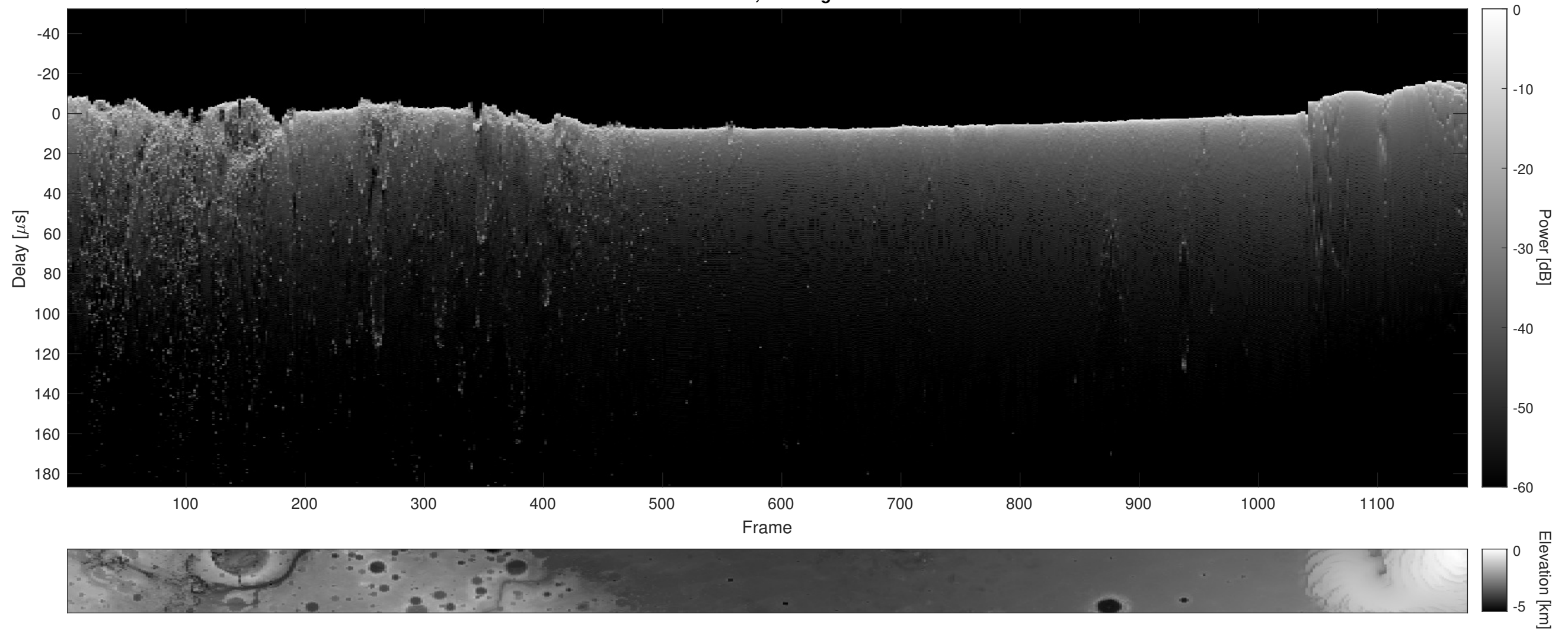
Orbit 5906, Cluttergram
