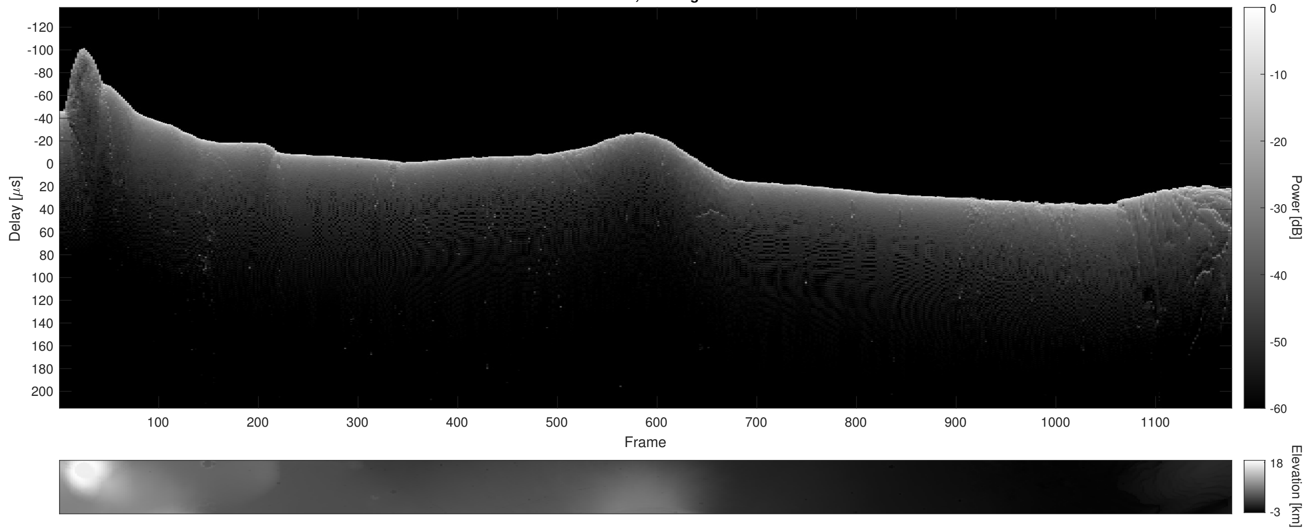
Orbit 5907, Cluttergram
