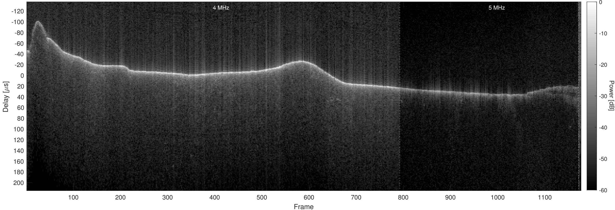
Orbit 5907, Optimized, No Window, Channel 2
