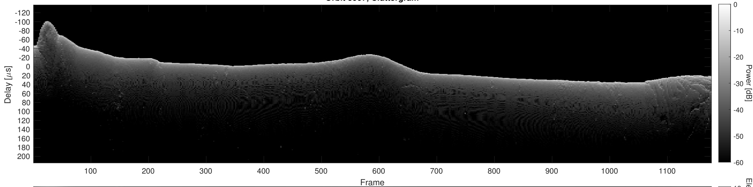
Orbit 5907, Cluttergram
