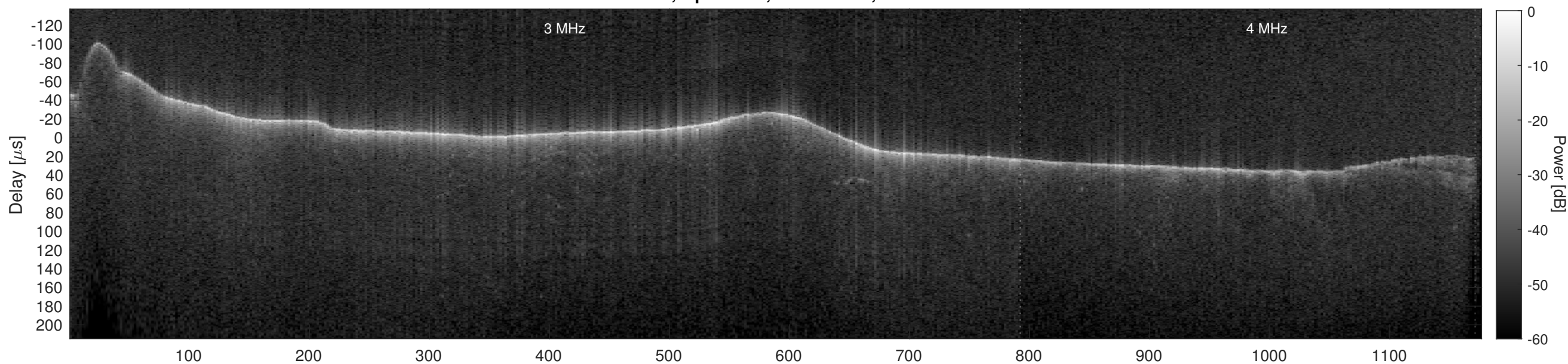
Orbit 5907, Cluttergram
