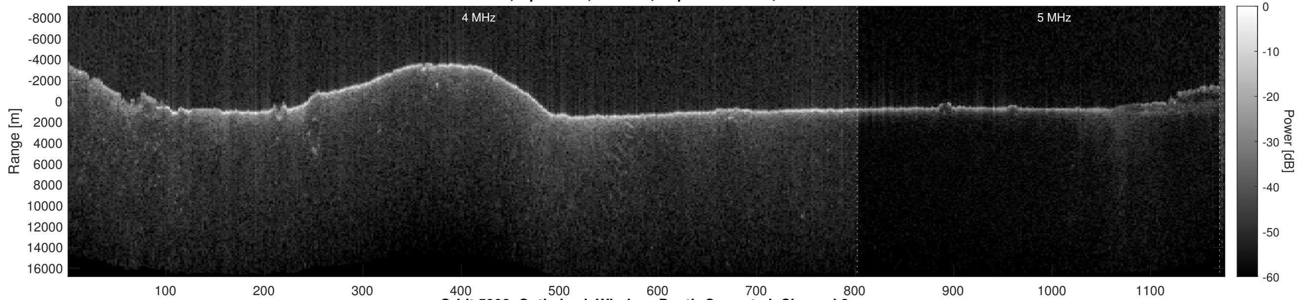
Orbit 5908, Optimized, Window, Depth-Corrected, Channel 2
