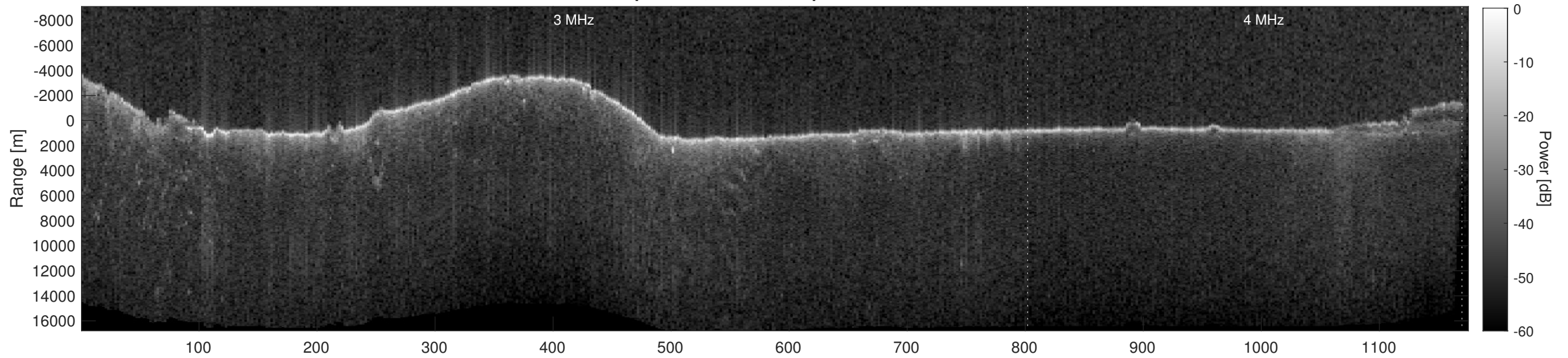
Orbit 5908, Depth-Corrected Cluttergram
