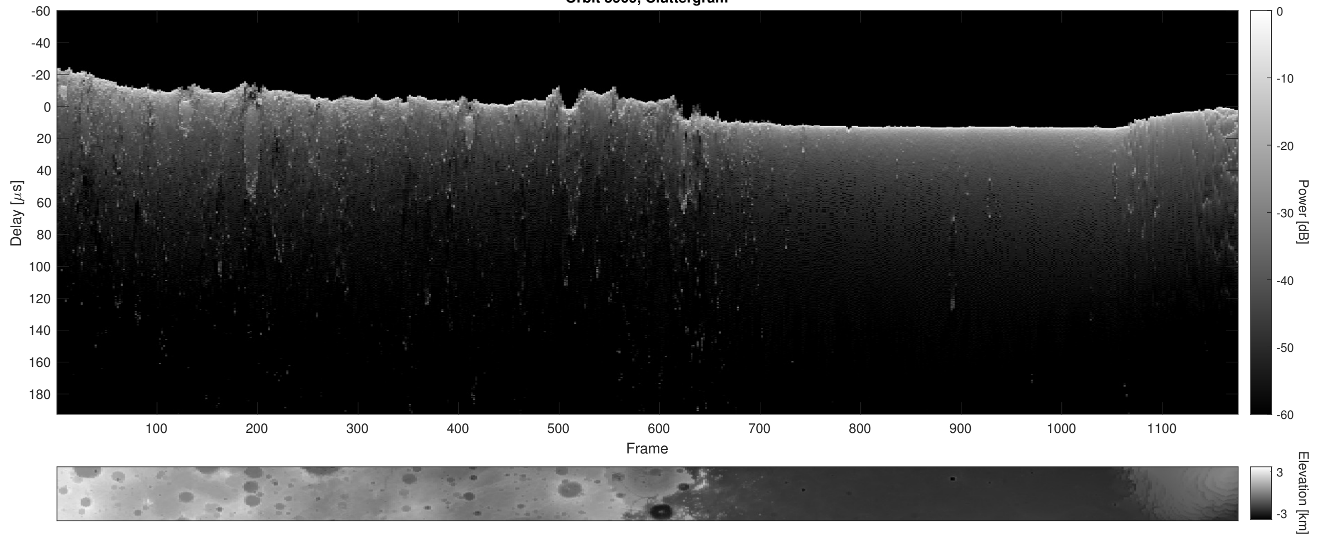
Orbit 5909, Cluttergram
