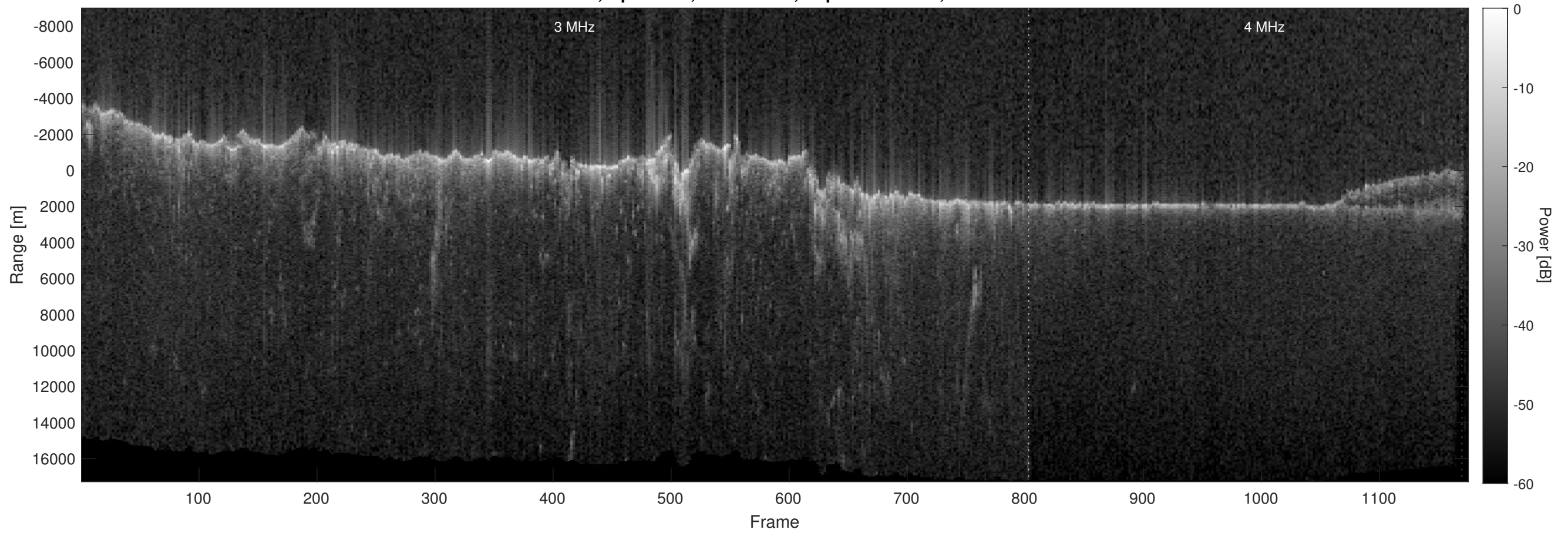
Orbit 5909, Optimized, No Window, Depth-Corrected, Channel 2
