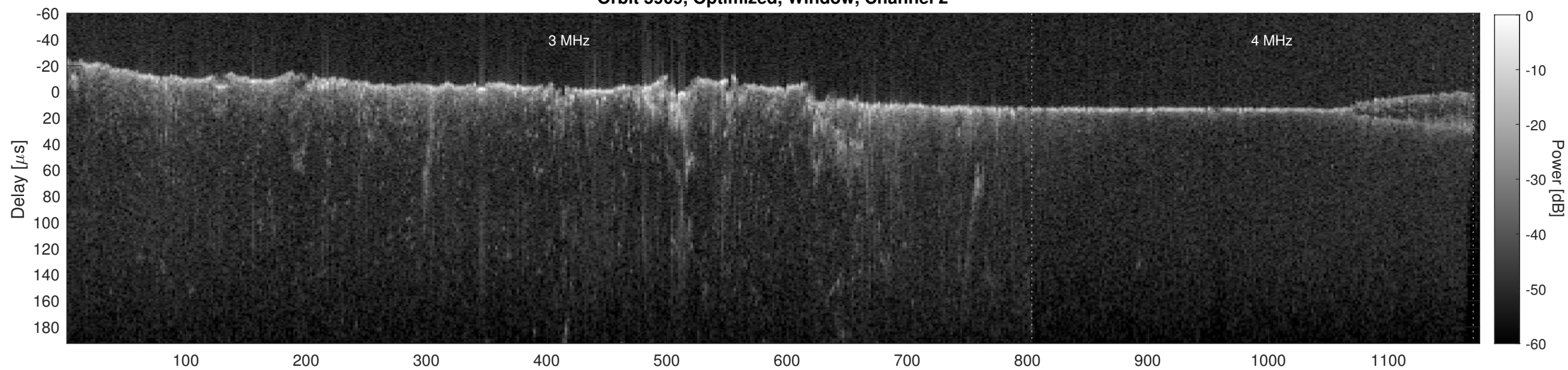
Orbit 5909, Cluttergram
