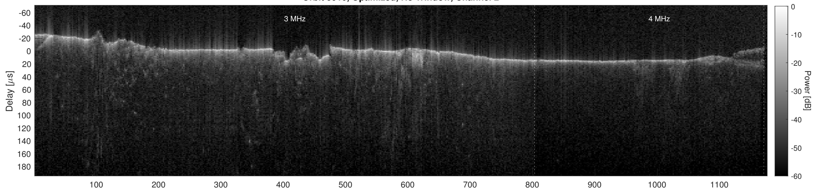
Orbit 5910, Cluttergram
