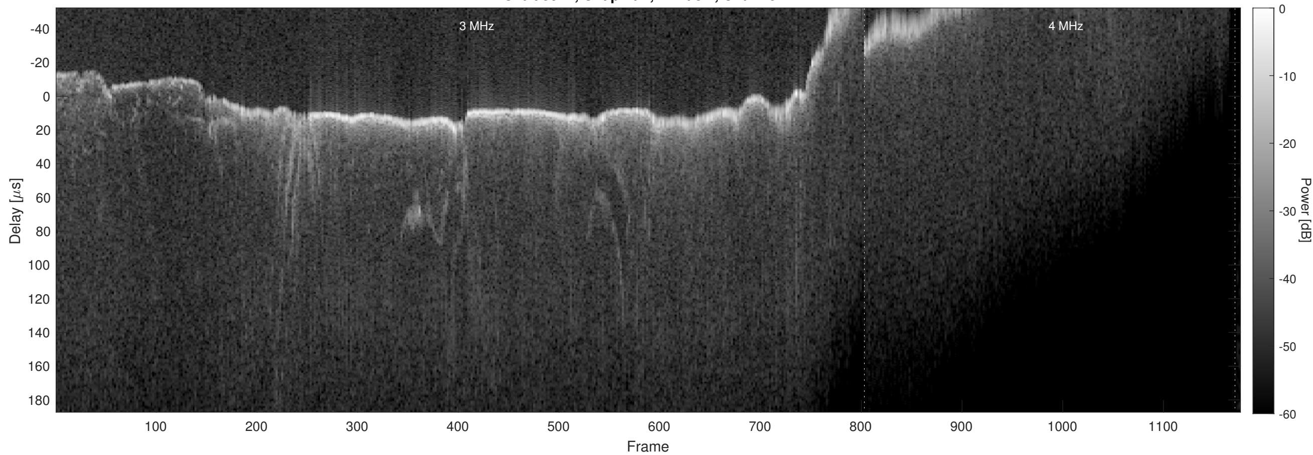
Orbit 5911, Chapman, Window, Channel 2
