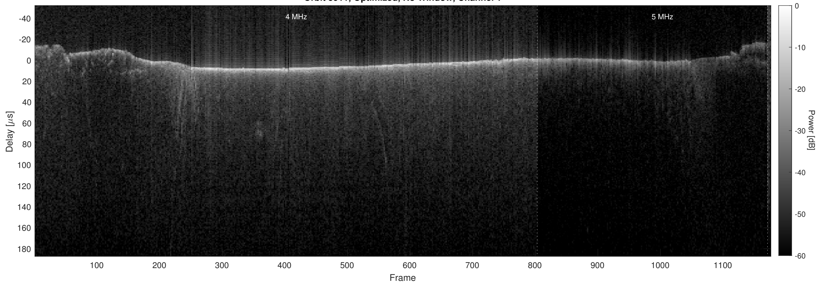
Orbit 5911, Optimized, No Window, Channel 2
