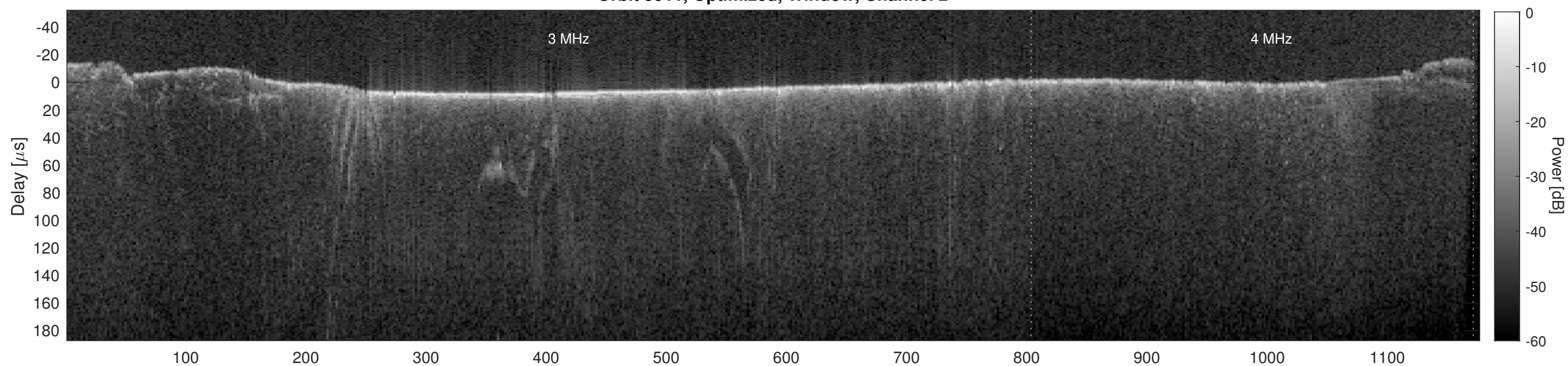
Orbit 5911, Cluttergram
