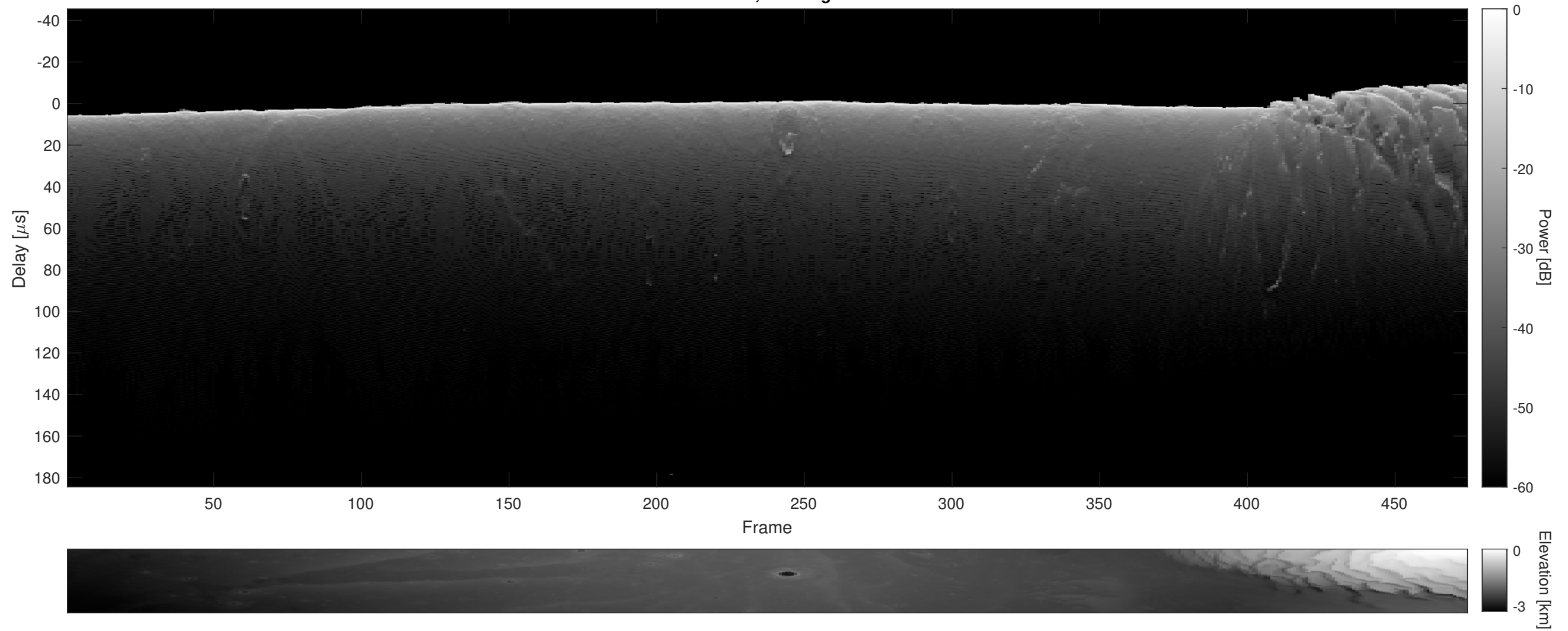
Orbit 5912, Cluttergram
