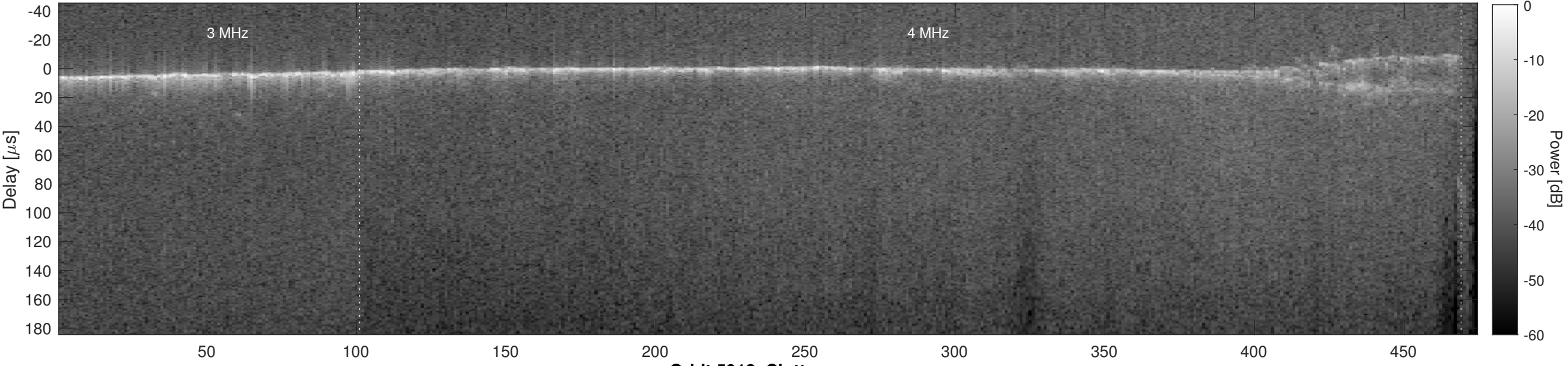
Orbit 5912, Cluttergram
