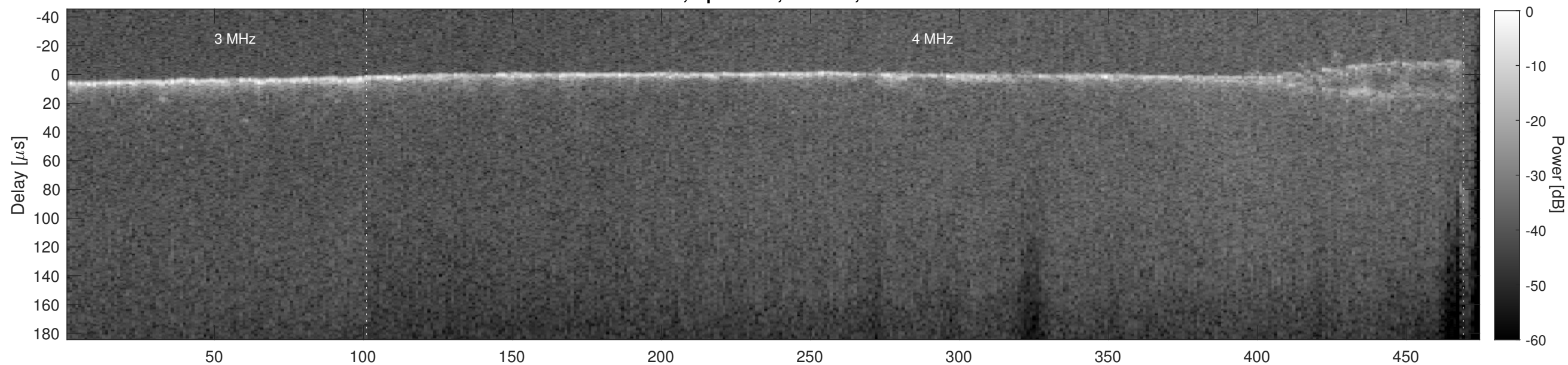
Orbit 5912, Cluttergram
