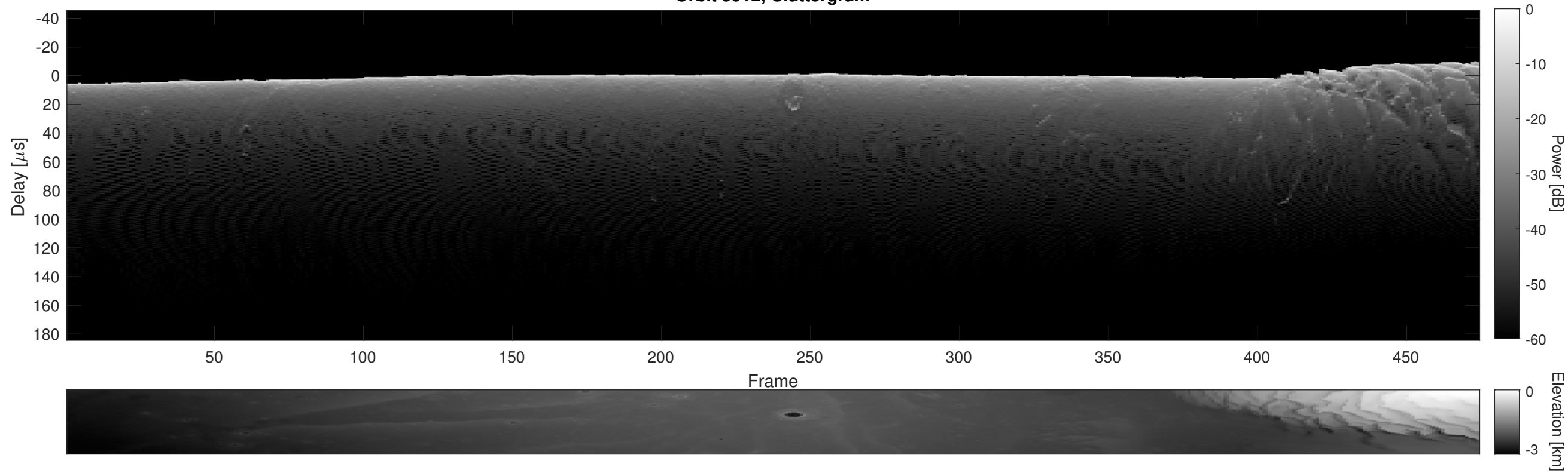
Orbit 5912, Cluttergram
