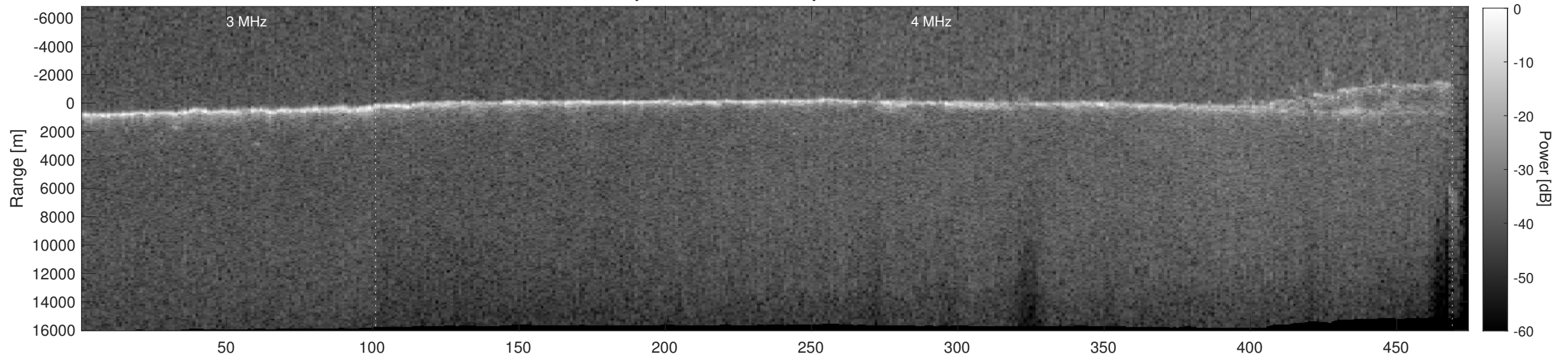
Orbit 5912, Depth-Corrected Cluttergram
