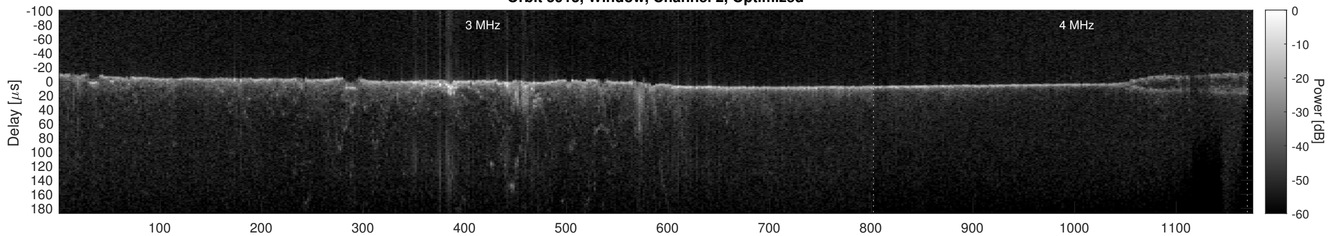
Orbit 5913, Cluttergram
