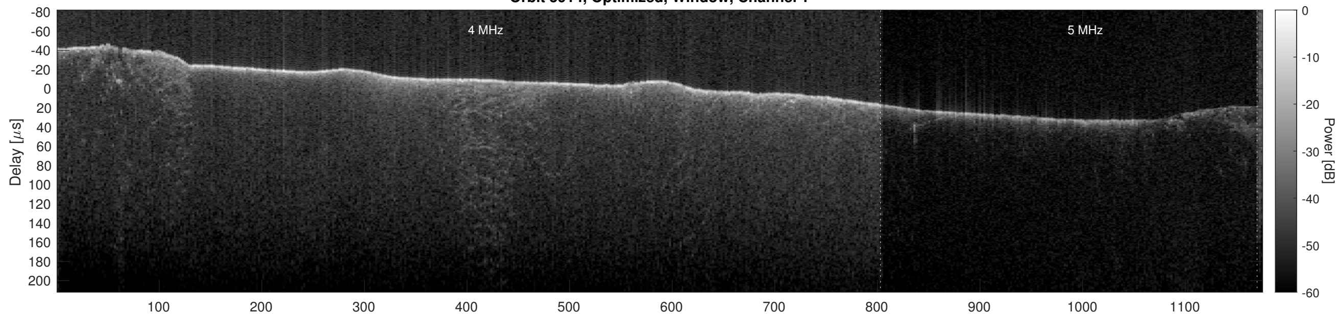
Orbit 5914, Optimized, Window, Channel 2
