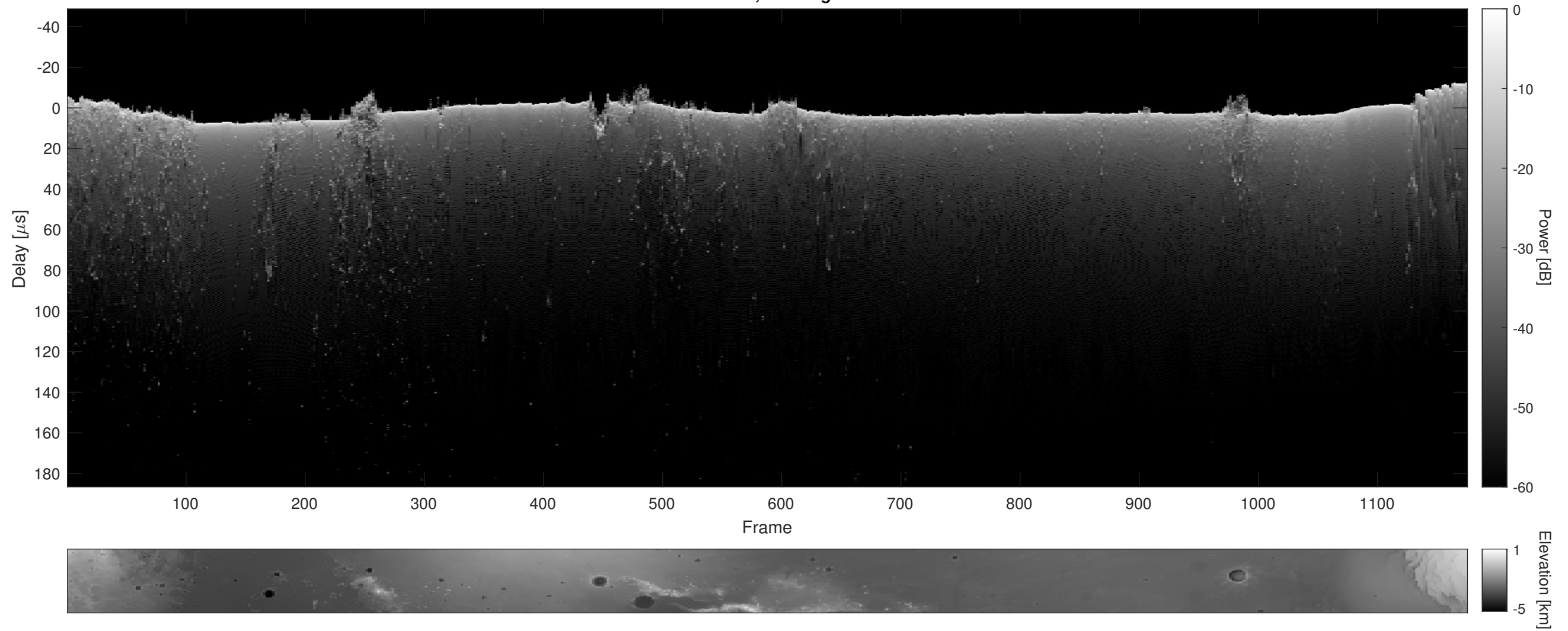
Orbit 5915, Cluttergram
