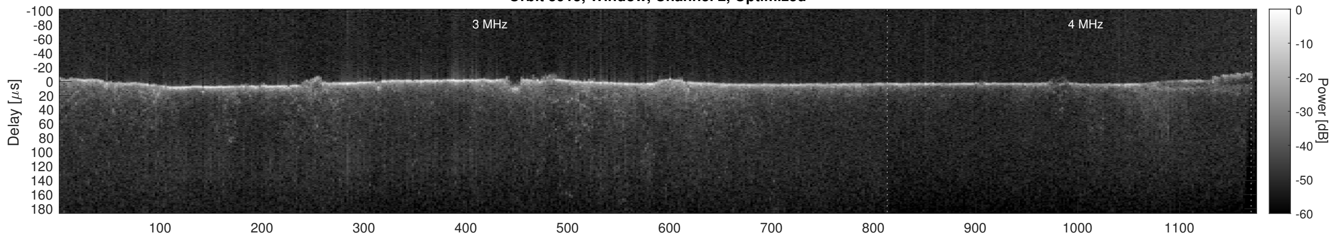
Orbit 5915, Cluttergram
