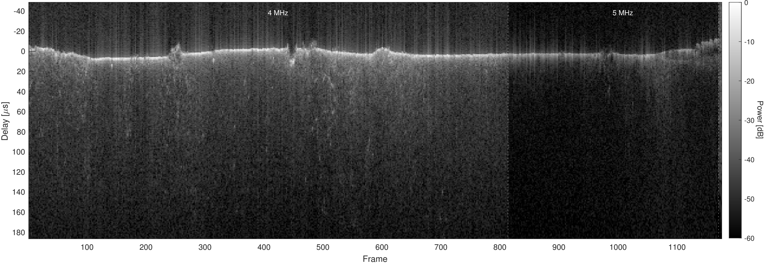
Orbit 5915, Optimized, No Window, Channel 2
