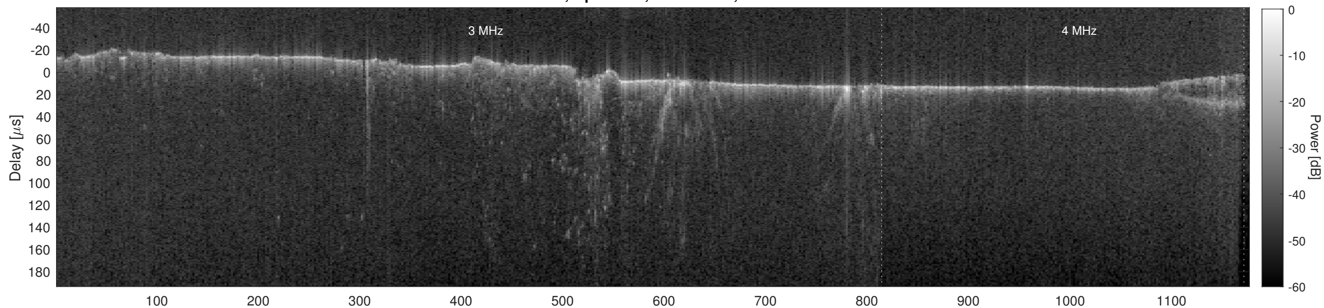
Orbit 5916, Cluttergram
