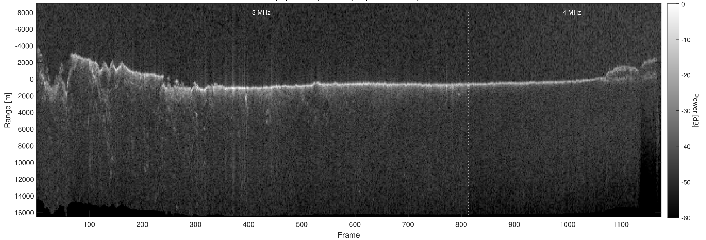
Orbit 5917, Optimized, Window, Depth-Corrected, Channel 2
