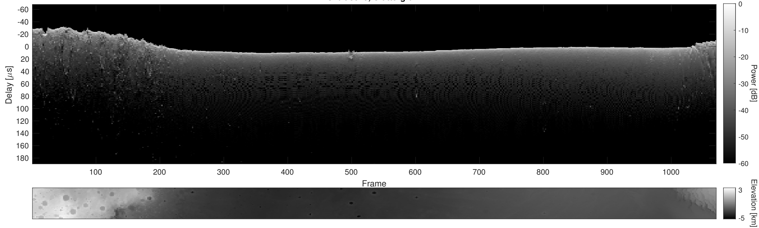
Orbit 5919, Cluttergram
