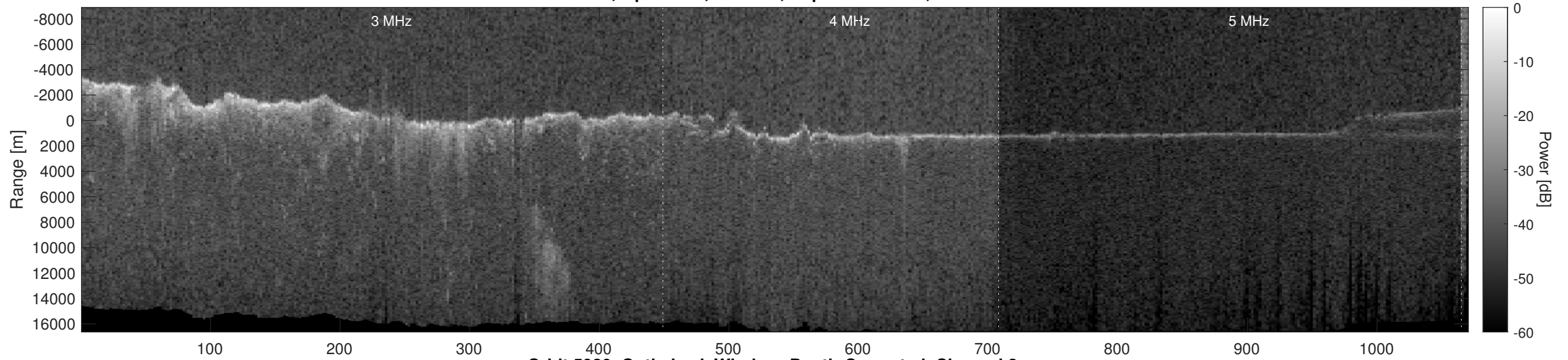
Orbit 5920, Optimized, Window, Depth-Corrected, Channel 2
