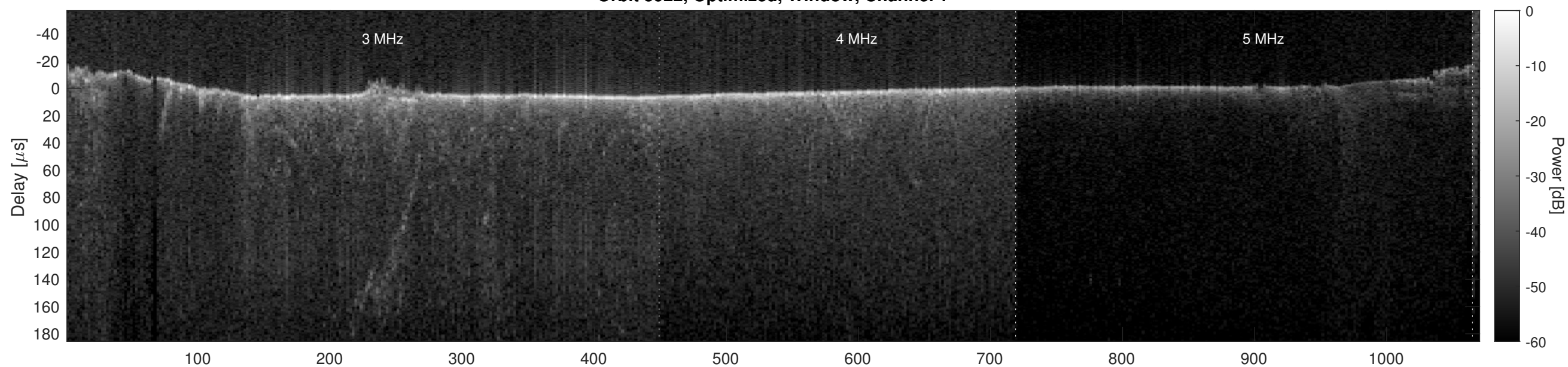
Orbit 5922, Optimized, Window, Channel 2
