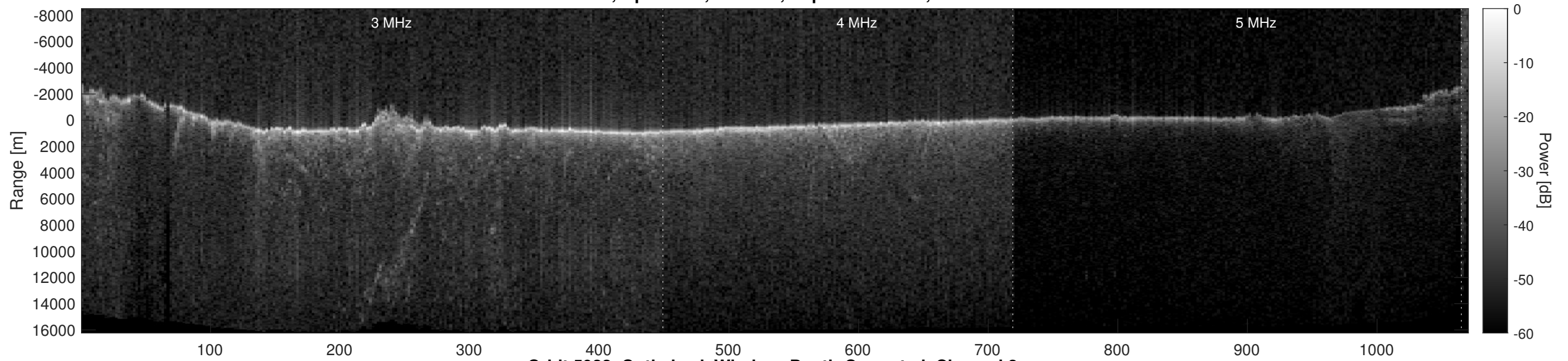
Orbit 5922, Optimized, Window, Depth-Corrected, Channel 2
