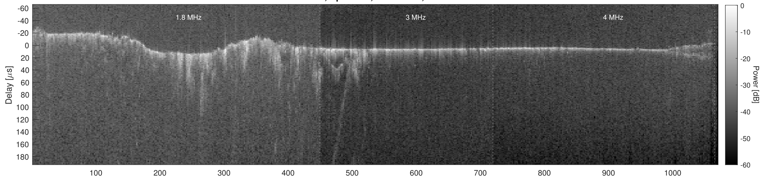
Orbit 5923, Cluttergram
