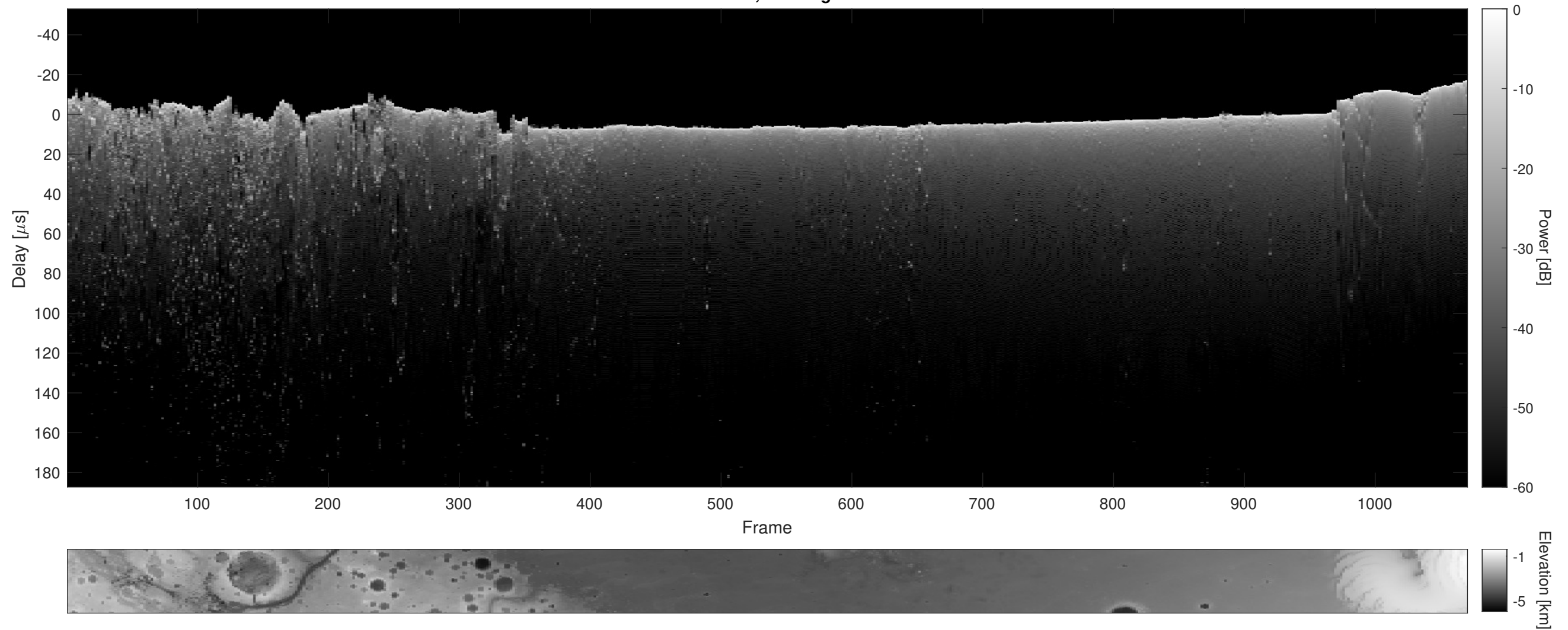
Orbit 5924, Cluttergram
