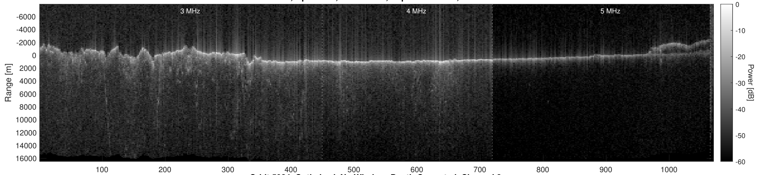
Orbit 5924, Optimized, No Window, Depth-Corrected, Channel 2
