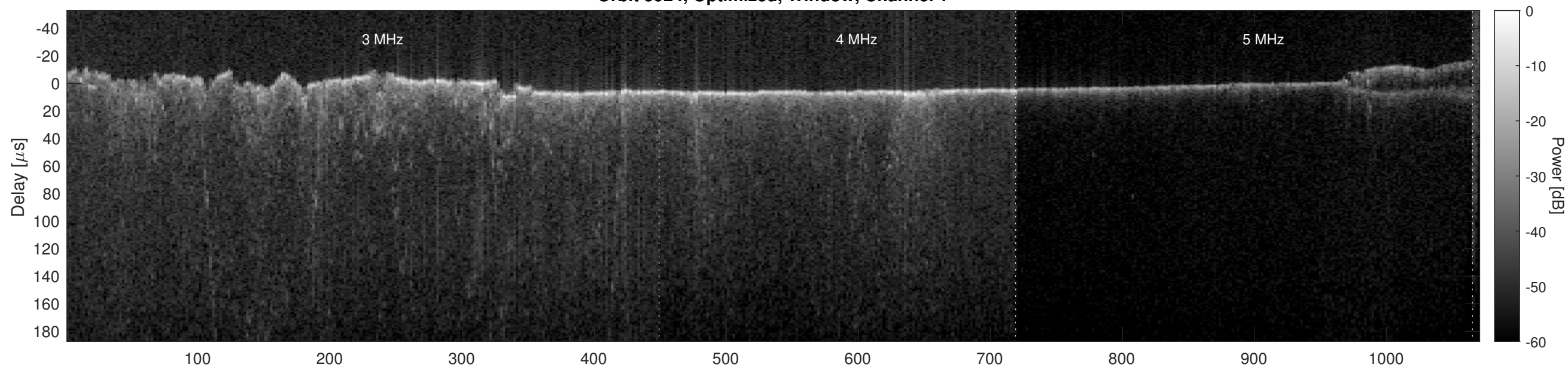
Orbit 5924, Optimized, Window, Channel 2
