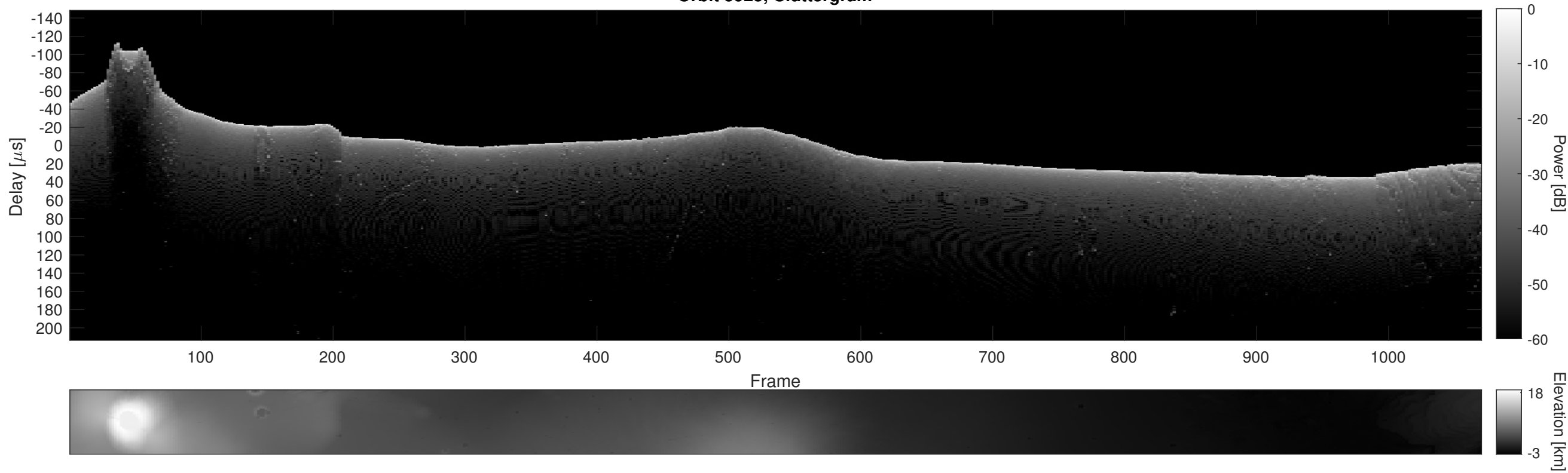
Orbit 5925, Cluttergram
