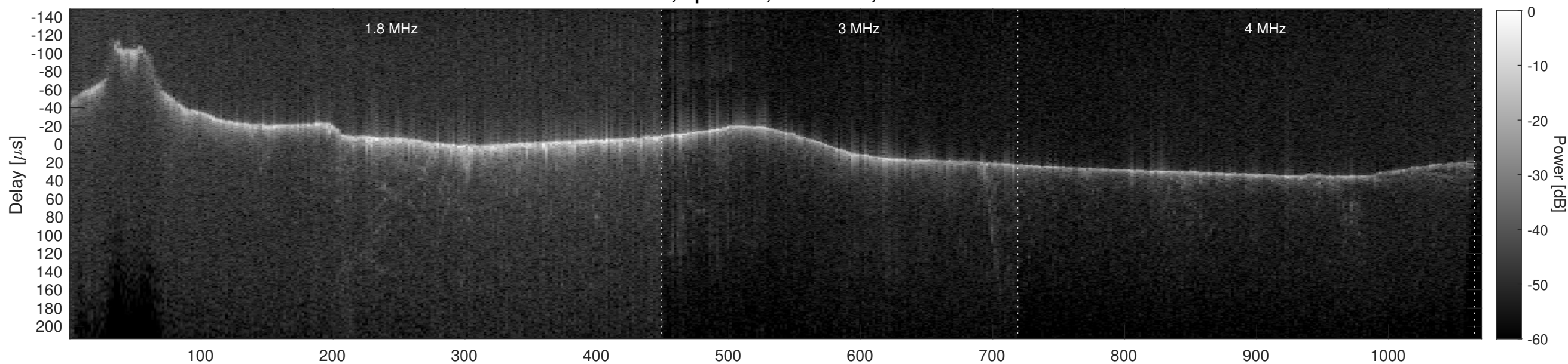
Orbit 5925, Cluttergram
