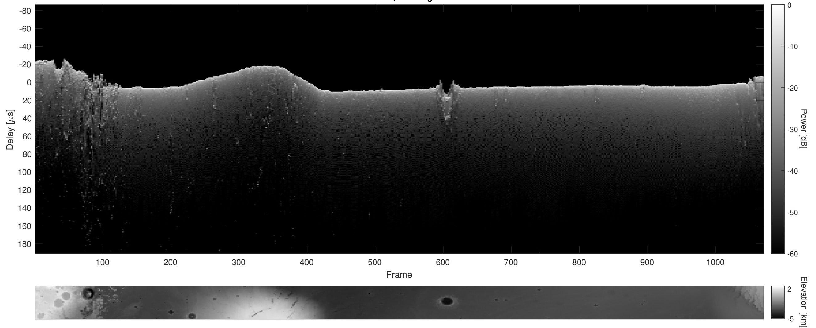
Orbit 5926, Cluttergram
