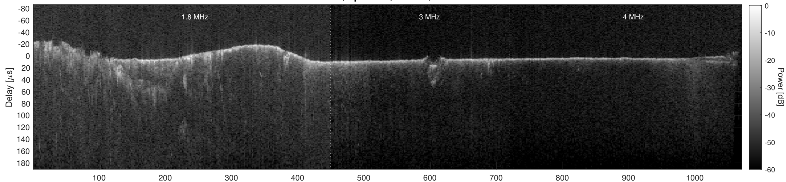
Orbit 5926, Cluttergram
