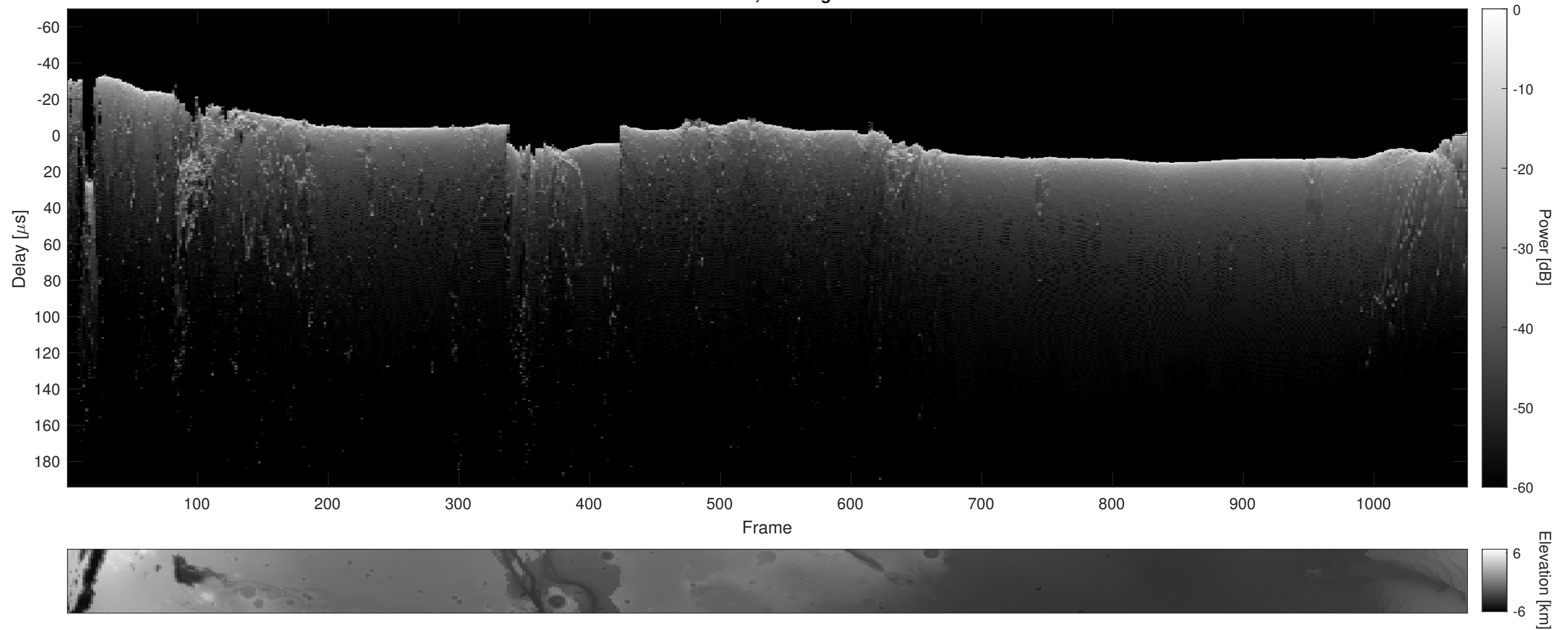
Orbit 5928, Cluttergram
