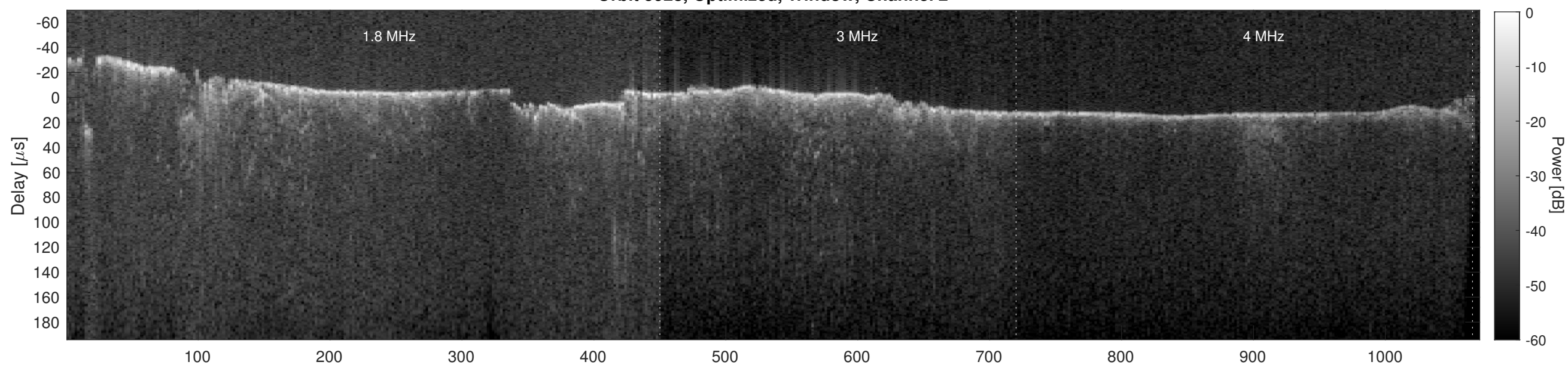
Orbit 5928, Cluttergram
