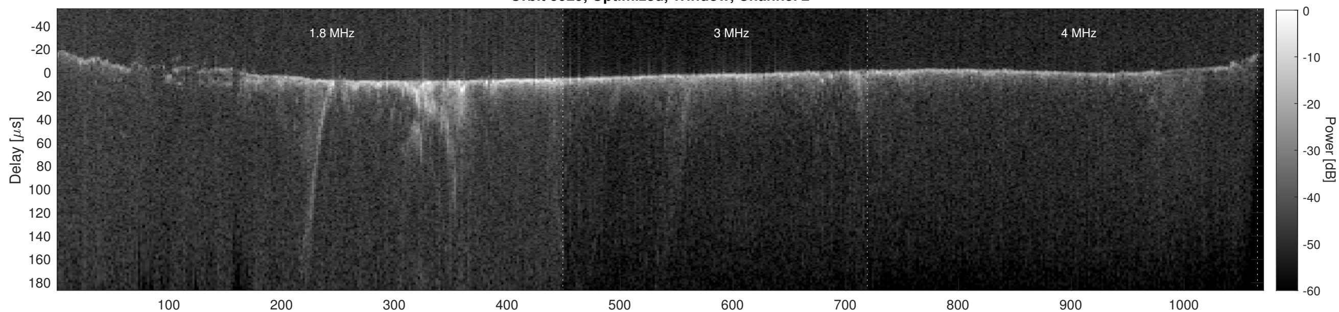
Orbit 5929, Cluttergram
