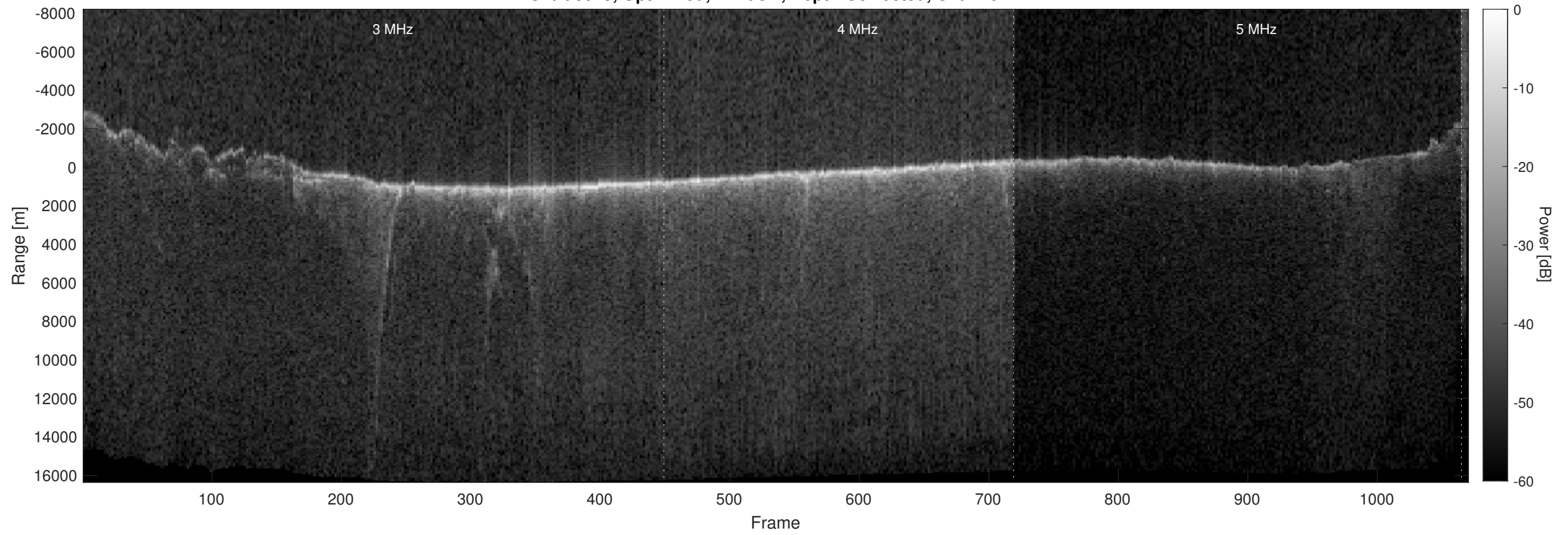
Orbit 5929, Optimized, Window, Depth-Corrected, Channel 2
