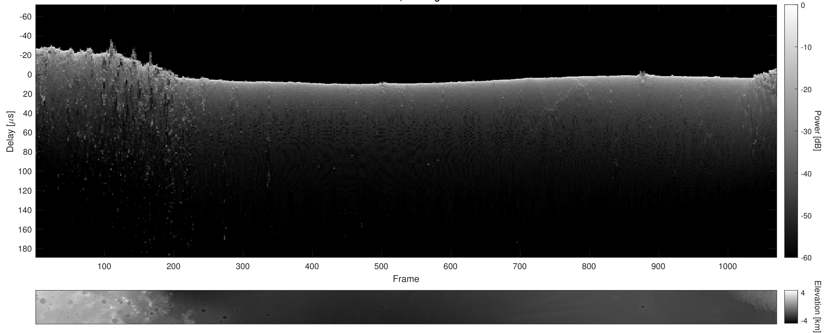
Orbit 5930, Cluttergram
