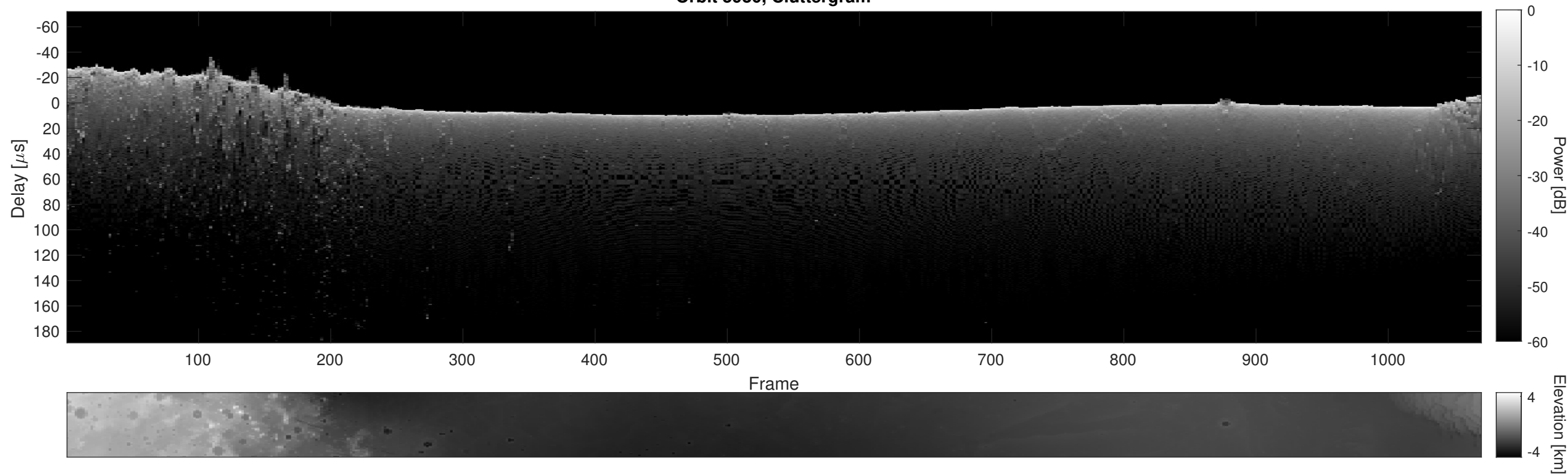
Orbit 5930, Cluttergram
