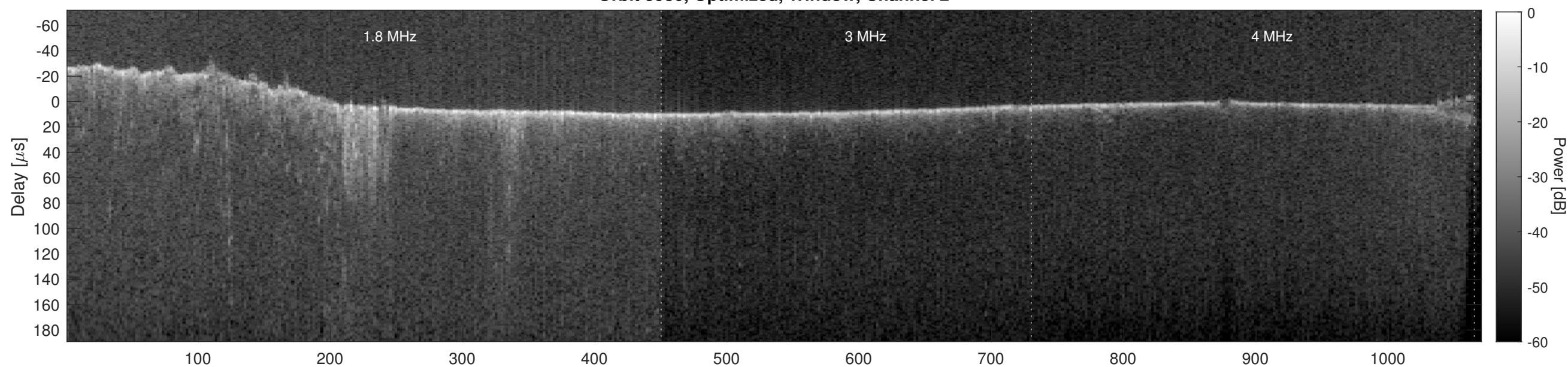
Orbit 5930, Cluttergram
