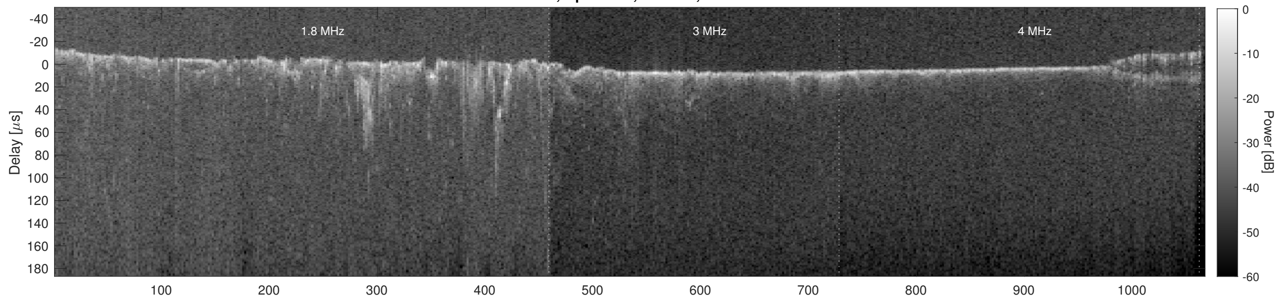
Orbit 5931, Cluttergram
